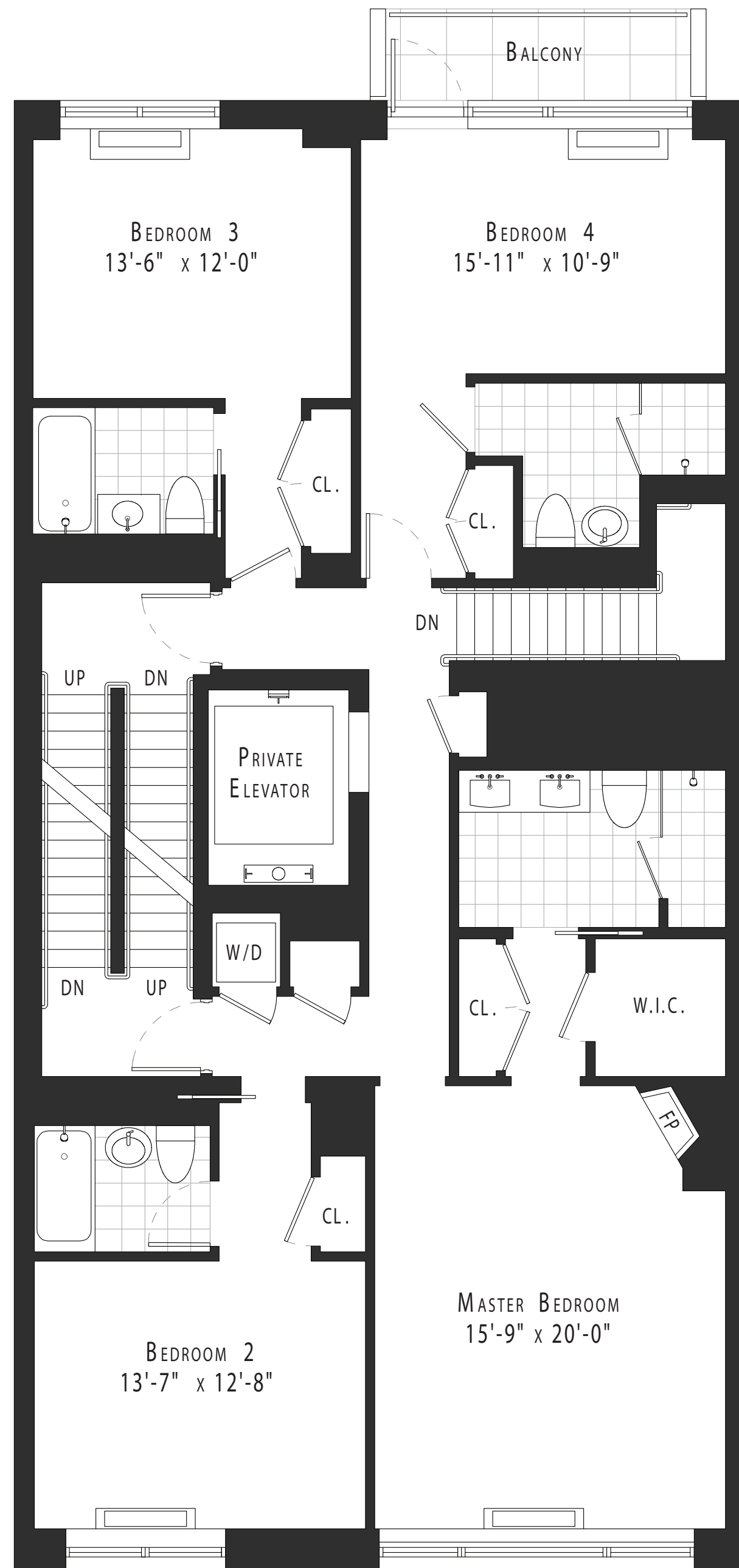
15TH FLOOR LOWER LEVEL PH PLAN
